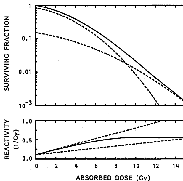
Figure 6. A superposition of two linear-quadratic relations (broken lines) which results in a seemingly exponential tail, i.e. a plateau of the reactivity, of the dose dependence for the mixed population (solid lines).
